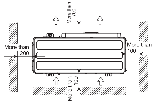
Service space
