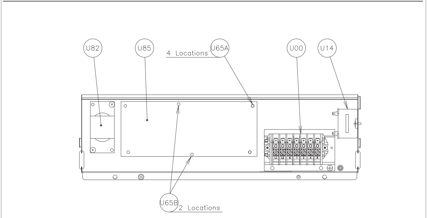
LOCATION OF ELECTRICAL EQUIPMENT IN THE ELECTRICAL CONTROL BOX
